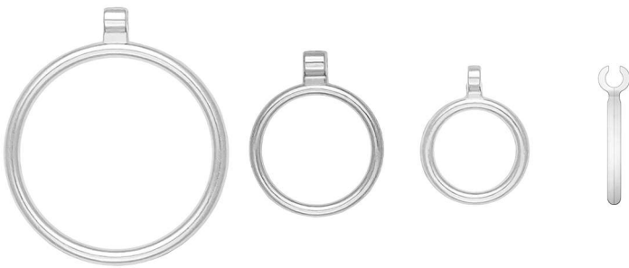
NMR406 CR5-8 NMR198 CR5 NMR202 CR3-5
